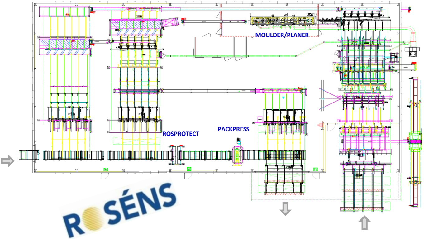
HIGH SPEED INFED TABLE TO THE MOULDER
